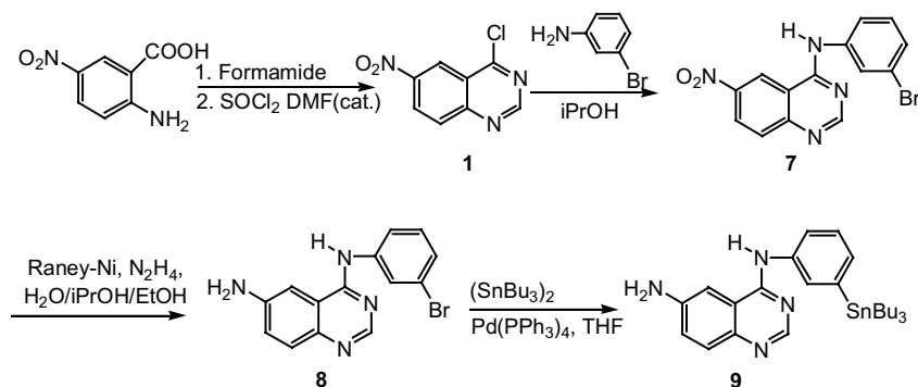
Figure 3. Synthesis of the starting material for radiolabeling with ^{124}\text{I} .
