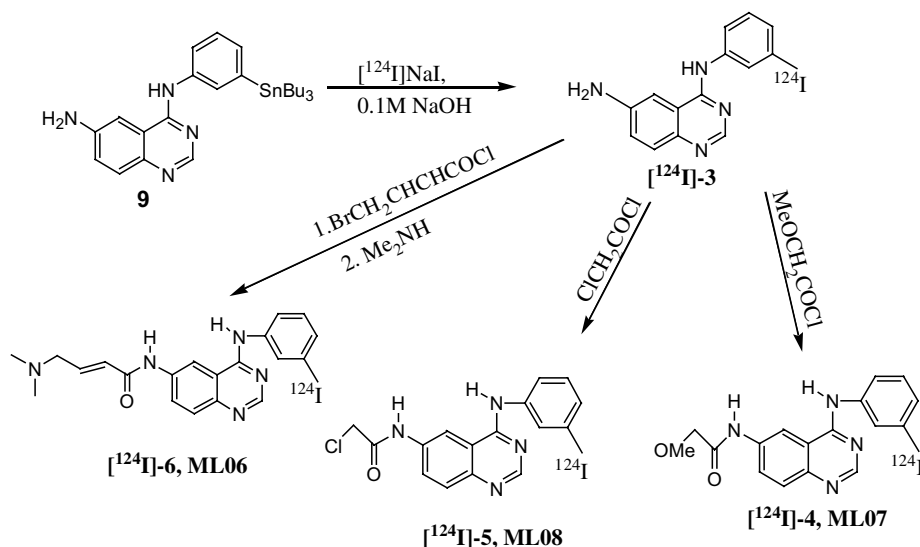
Figure 4. ^{124}\text{I} labeling of irreversible EGFR inhibitors.
