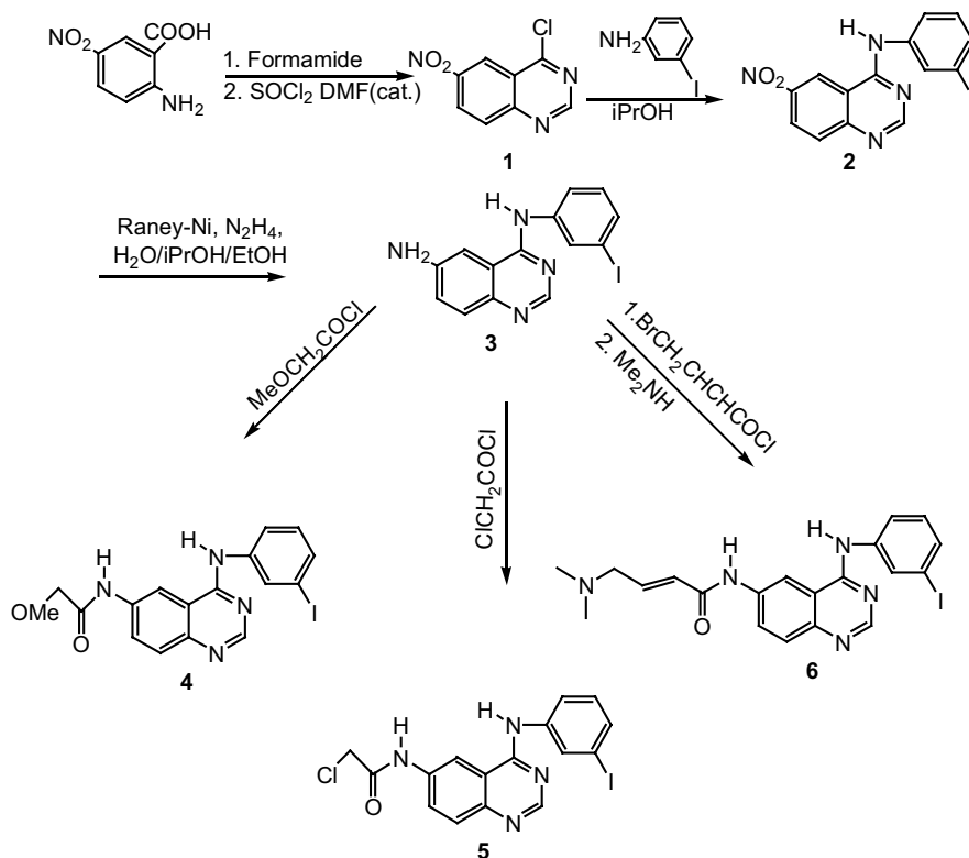
Figure 2. Synthesis of new irreversible EGFR inhibitors.
