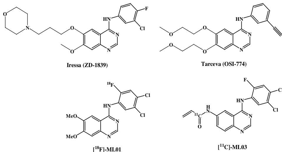
Figure 1. Chemical structure of reversible and irreversible EGFR inhibitors.
